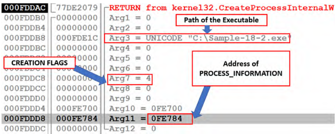
Figure 18-11. Stack displaying the parameters of CreateProcessInternalW
