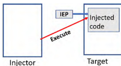
Figure 18-1. Injection process and the injection entry point
