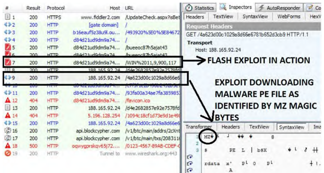
Figure 6-6. HTTP communication shows a successful exploitation and malware download
