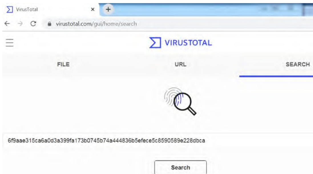
Figure 12-4. Querying VirusTotal using the sha256 hash for Sample 12-1
