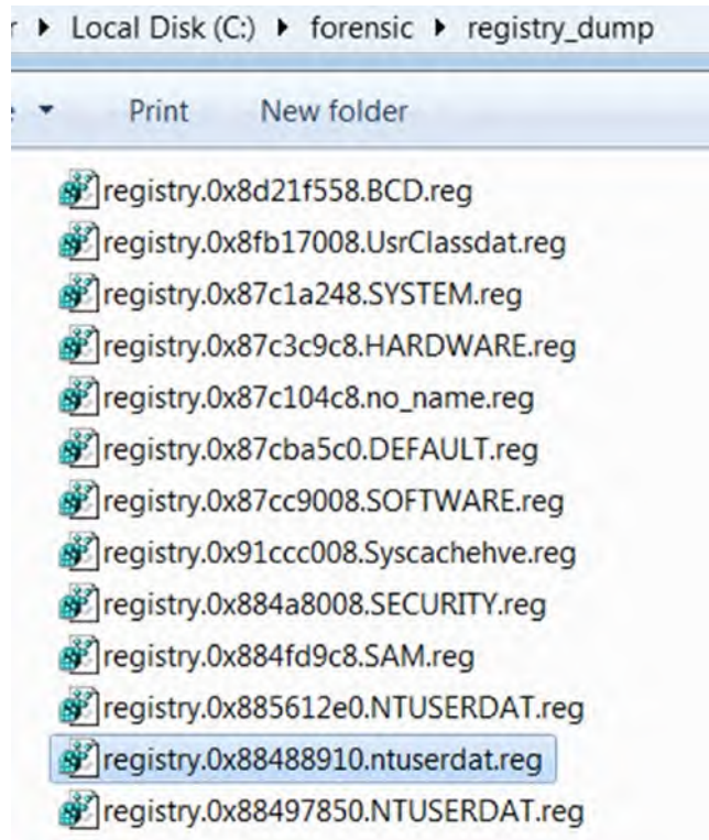
Figure 14-20. The registry hives dumped as files using the dumpreistry Volatility command
