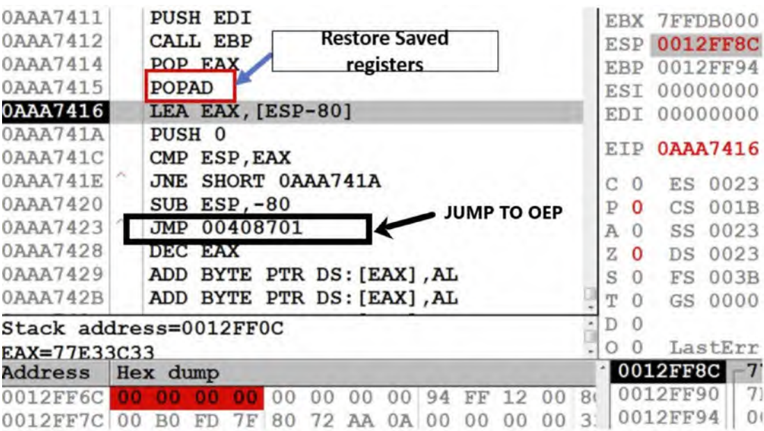
Figure 17-9. Debugger breaks on hardware breakpoint we have set on Sample-17-2.exe
