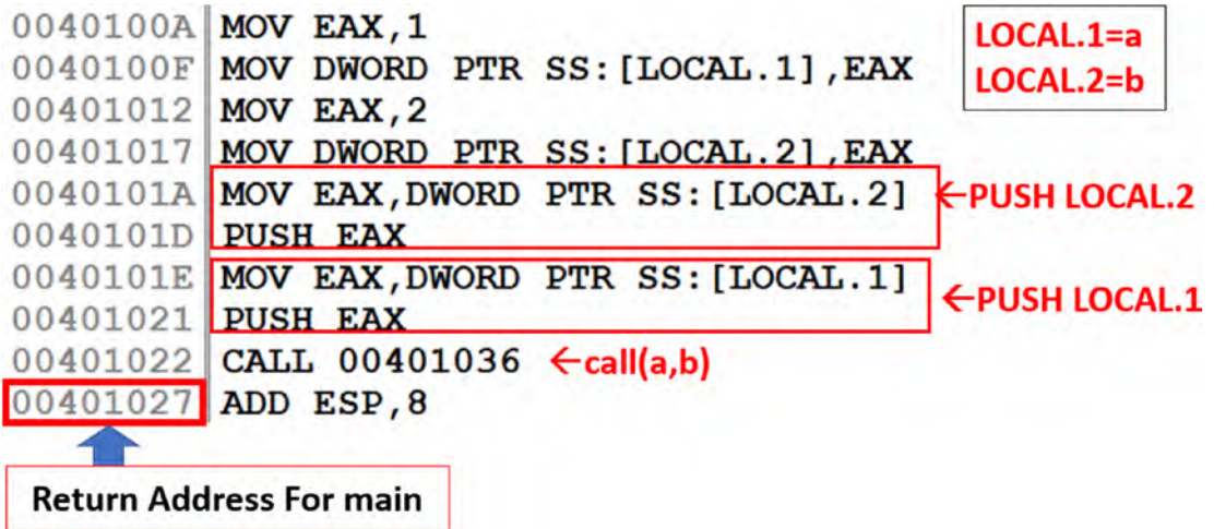
Figure 16-50. Parameters passed from main() to sum() in the main() function of Sample-16-9 corresponding to its C code in Listing 16-24
