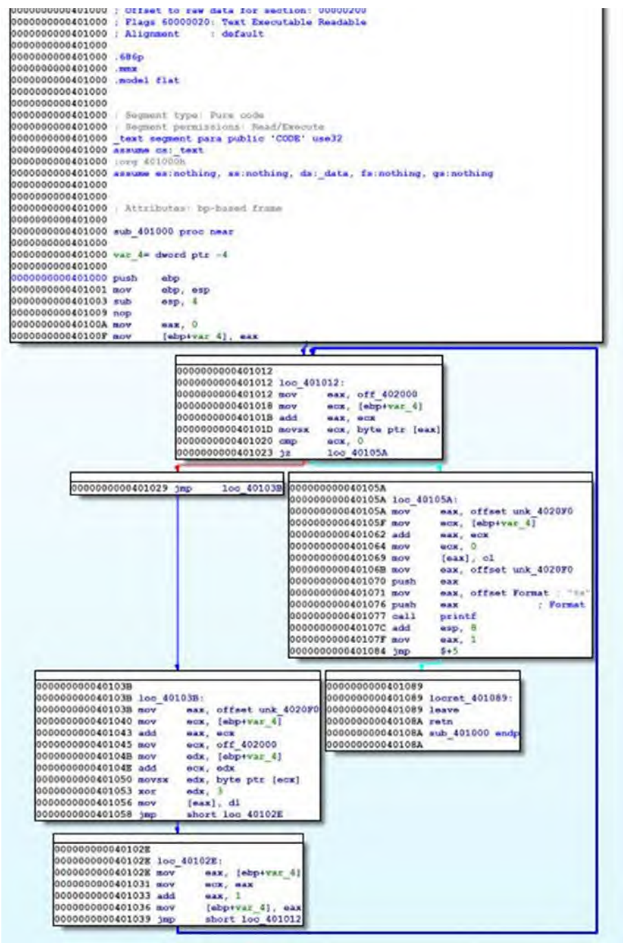
Figure 16-63. IDA graph view for the main() function of Sample-16-2
