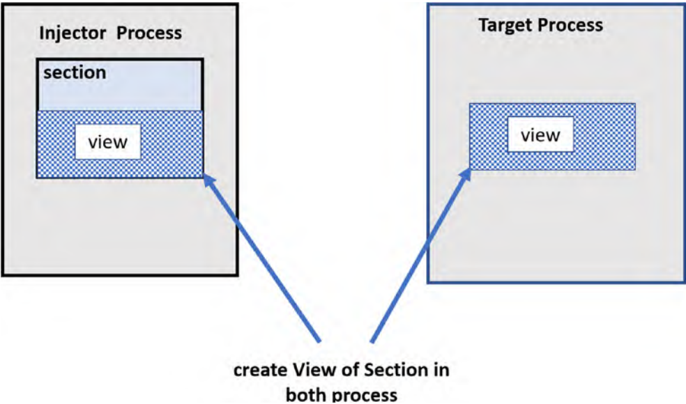
Figure 10-15. View of a section in both the Injector and target process
