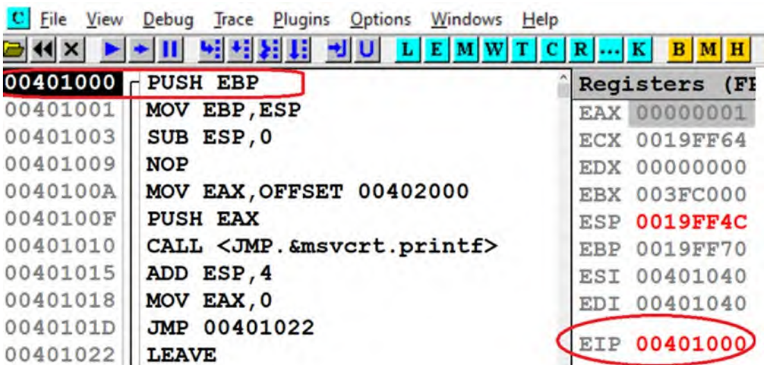
Figure 16-24. Result of stepping into the CALL instruction at 0x40109E of Sample-16-1 (also seen in Figure 16-23)
