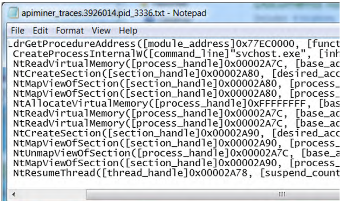
Figure 13-8. APIMiner API logs for Sample-13-1 shows a malicious sequence of APIs
