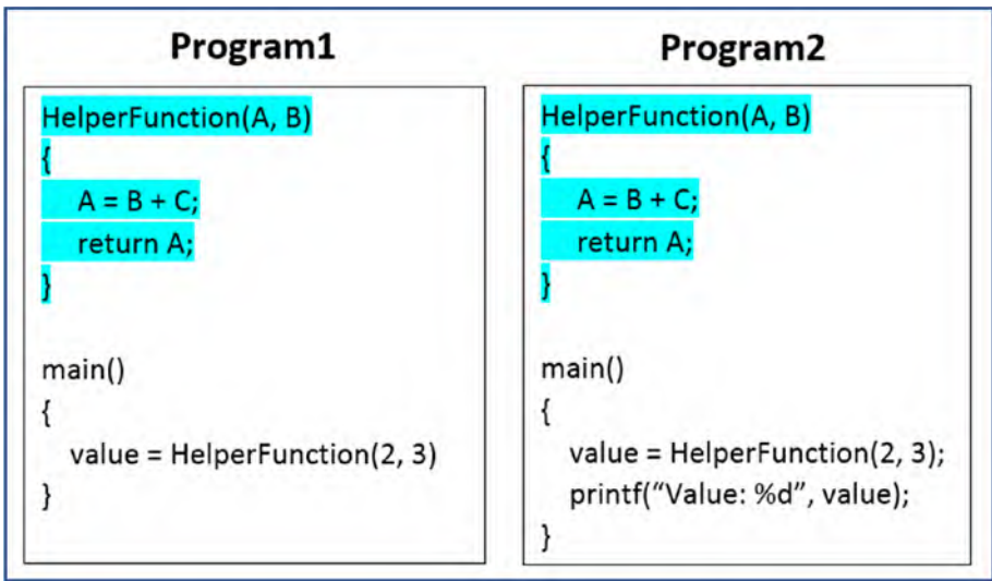
Figure 4-34. 2 C Programs that each have a HelperFunction() defined that are exact replicas
