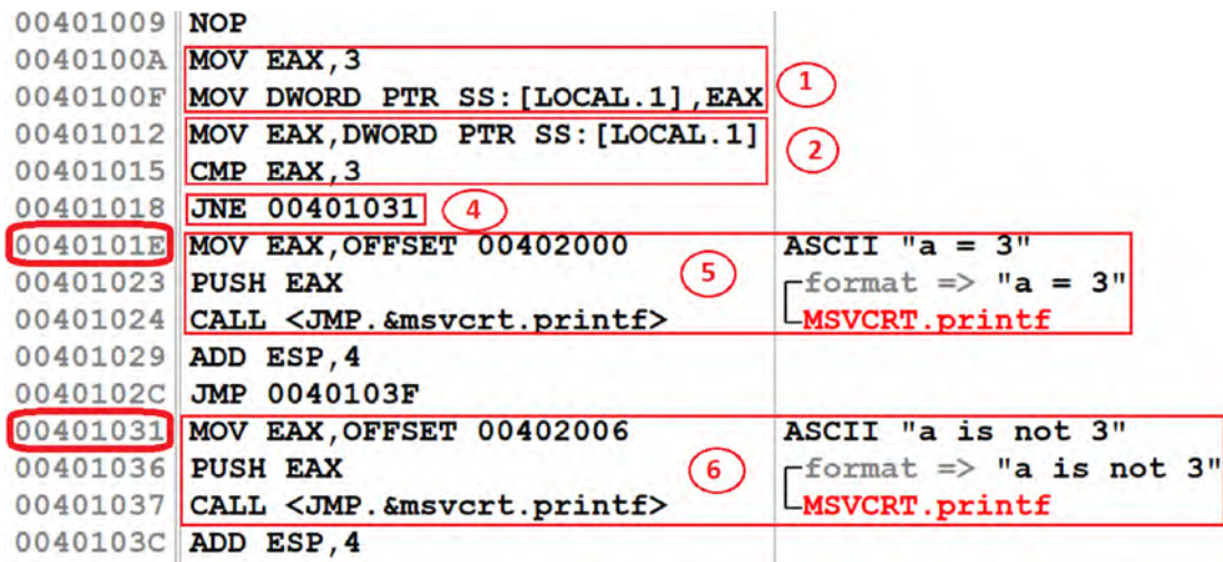
Figure 16-53. Disassembly of the main() function in Sample-16-10 that shows conditional checks and jumps
