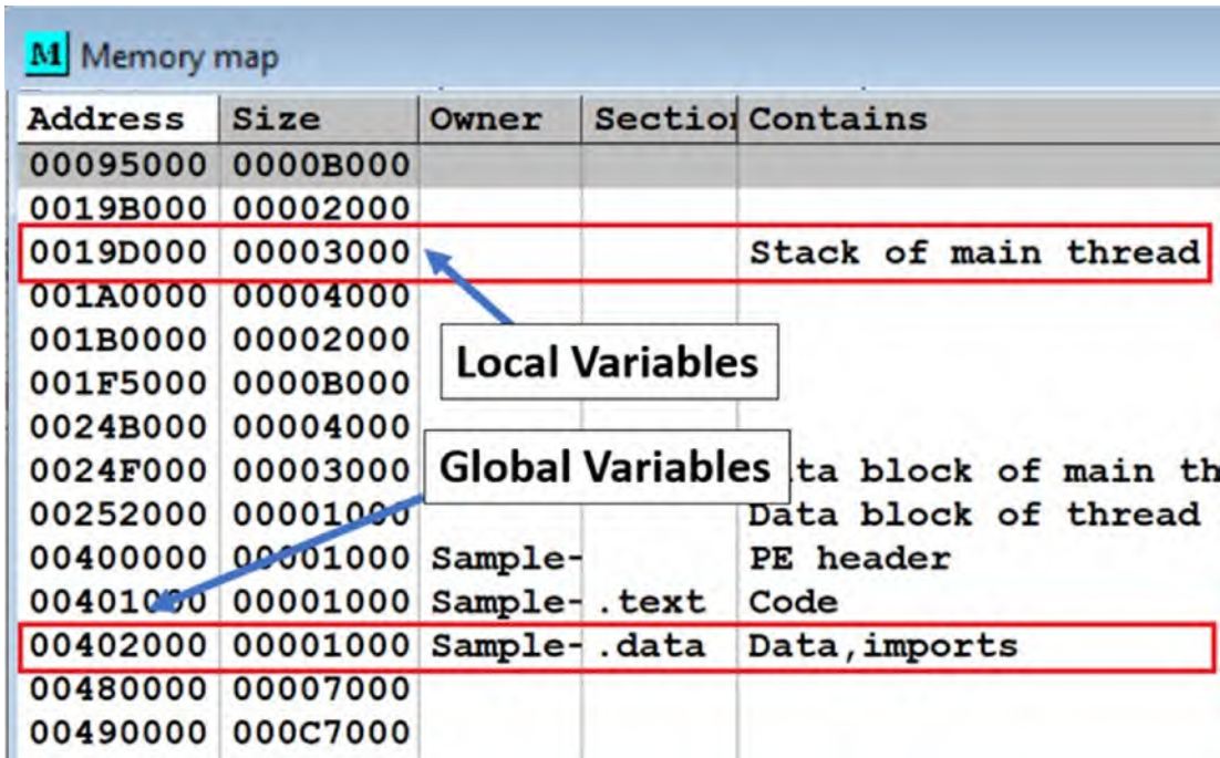
Figure 16-46. The Memory map window shown by OllyDbg for Sample-16-6 that clearly shows the memory blocks used by the stack that hold the local variables
