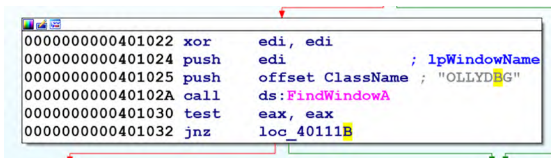
Figure 19-2. FindWindow API used by the malware Sample-19-2 as an armoring technique, to detect the presence of OllyDbg process on the system
