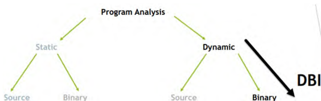
Figure 25-1. Categorization of different types of program analysis and where DBI lies in it
