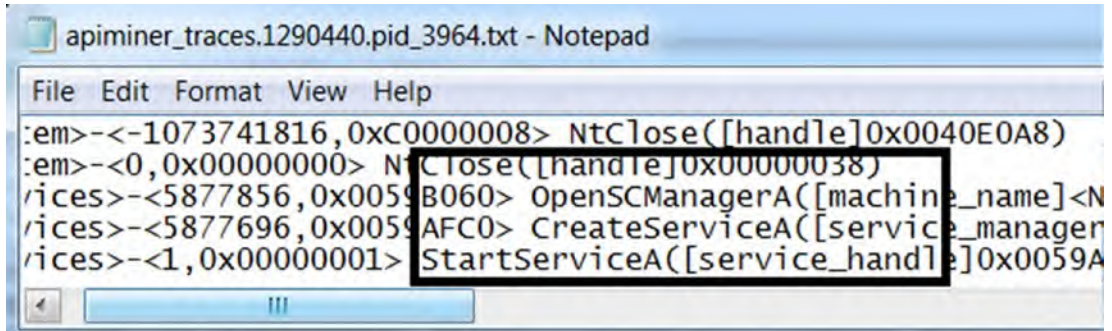
Figure 11-37. API sequence indicates the sample is creating and starting a service.
