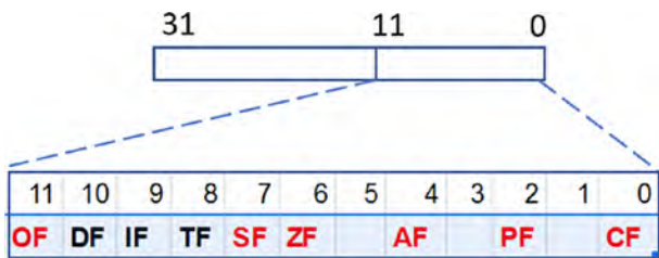
Figure 16-11. eflags register
