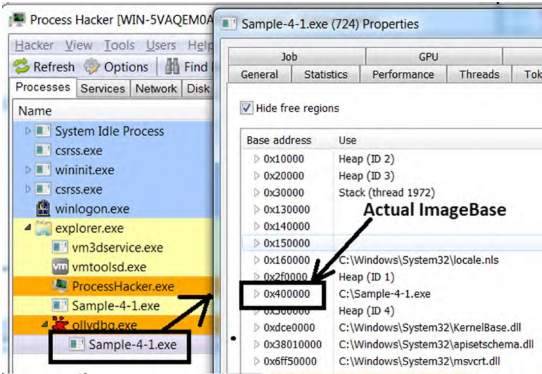
Figure 4-25. The actual image base of Sample-4-1.exe PE file in its memory
