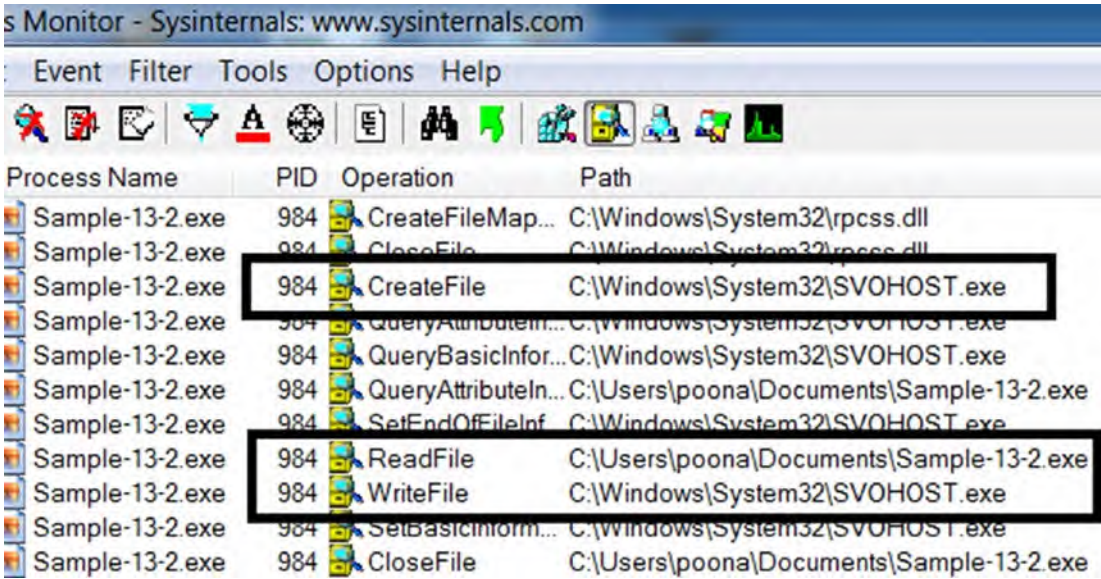
Figure 13-18. ProcMon events show the sample copying itself into system folder as a new file SVCHOST.EXE
