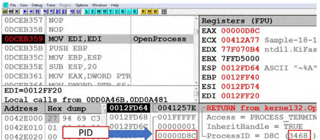
Figure 18-3. Debugger breaks at OpenProcess API on which we have set a breakpoint for Sample-18-1.exe
