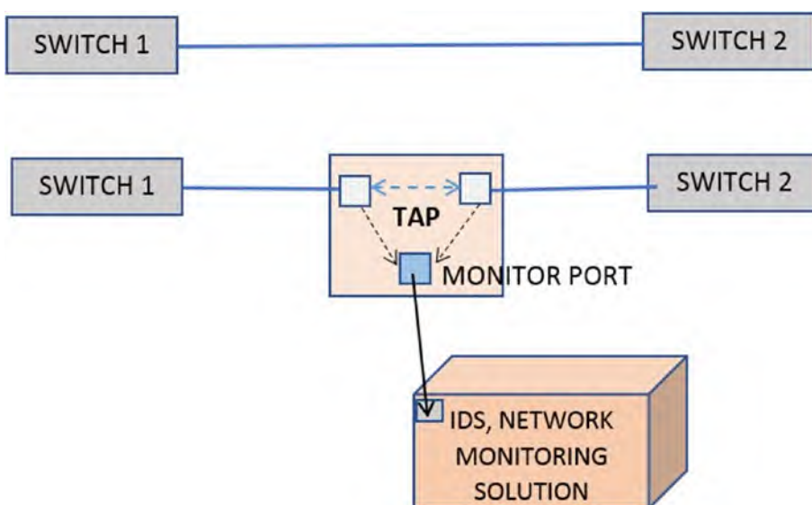
Figure 23-3. TAP copying packets into its monitor port which can then be fed into IDPS
