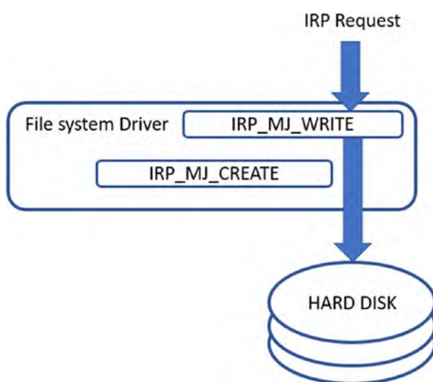
Figure 11-39. Flow of IRP across the file system driver which then operates on the disk
