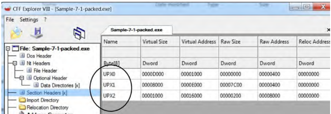
Figure 7-18. Section names for UPX packed files that start with the string UPX
