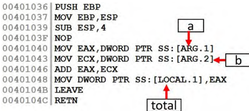
Figure 16-51. The sum() function in Sample-16-9 that shows the parameters passed to it
