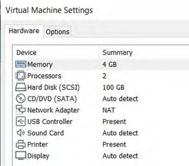
Figure 21-1. Hardware settings for the dev VM with VMWare workstation
