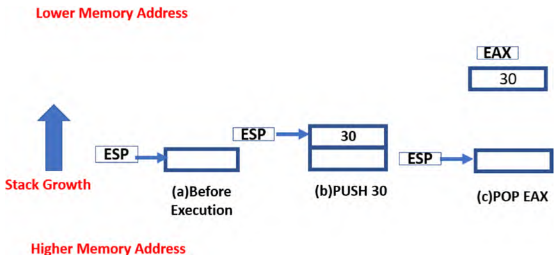
Figure 16-12. Illustration of how the stack grows when data is pushed and popped from it
