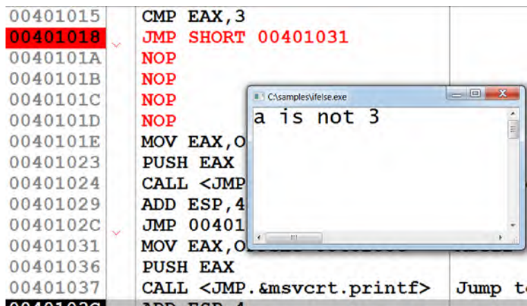
Figure 16-83. Executing Sample-16-17 after patching its instruction at 0x401018 into an unconditional jump instruction
