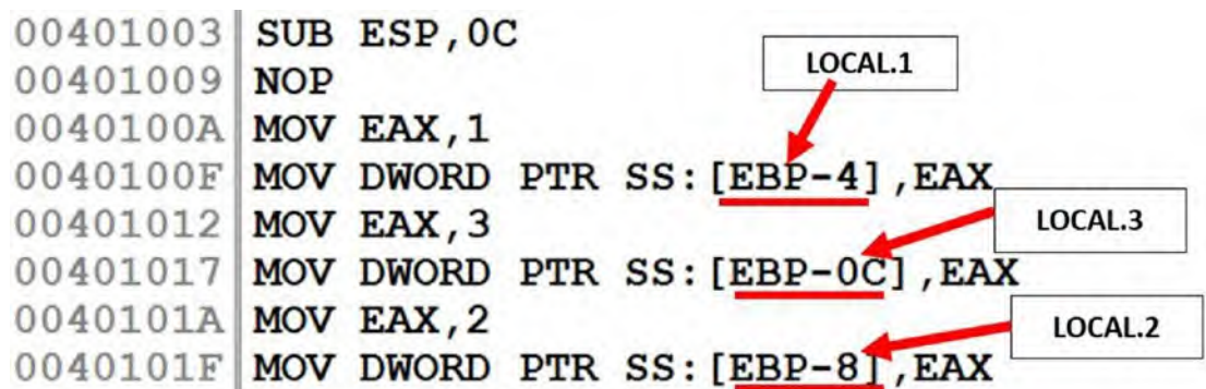
Figure 16-42. Actual disassembly for LOCAL.1, LOCAL.2 and LOCAL.3 seen after removing analysis
