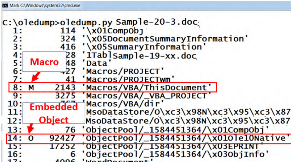
Figure 20-15. oledump.py tool to view OLE file format of Sample-20-3.doc
