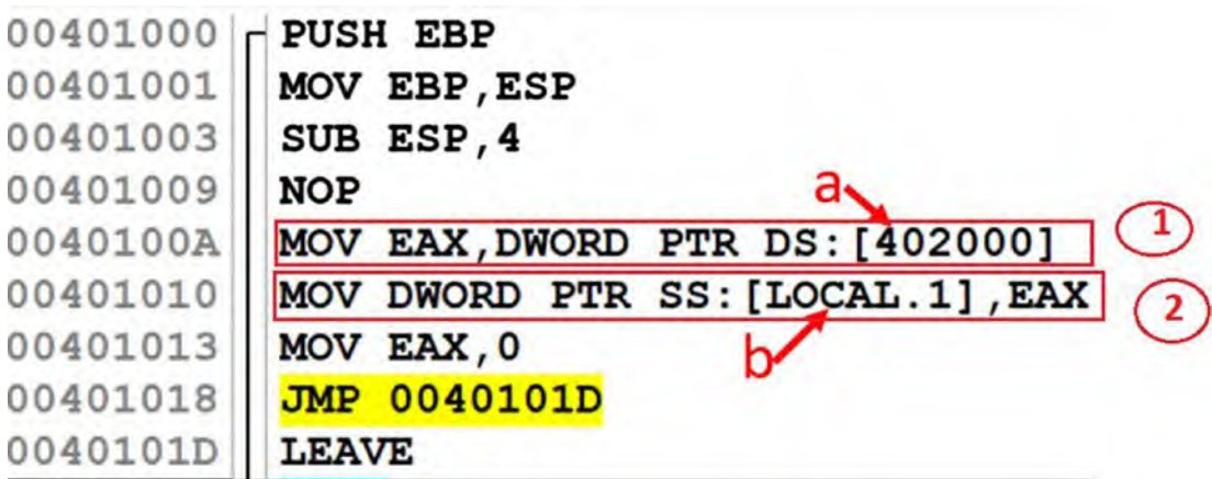
Figure 16-45. Disassembly of the main() function in Sample-16-6 that shows global vars
