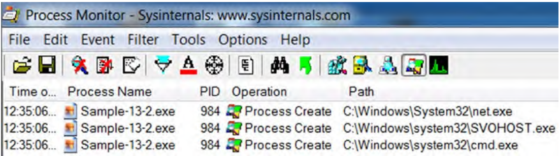
Figure 13-21. Process creation events from ProcMon shows Sample-13-2.exe creating a new process out of SVOHOST.exe which it created earlier in the Windows system folder
